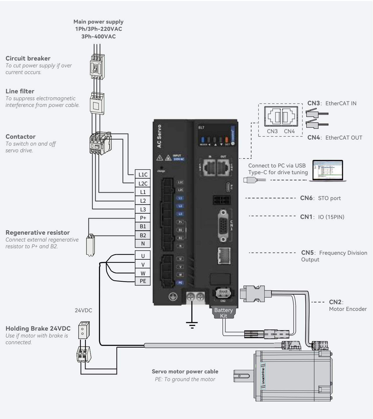
EL7-ECN & Peripheral Wiring Diagram
