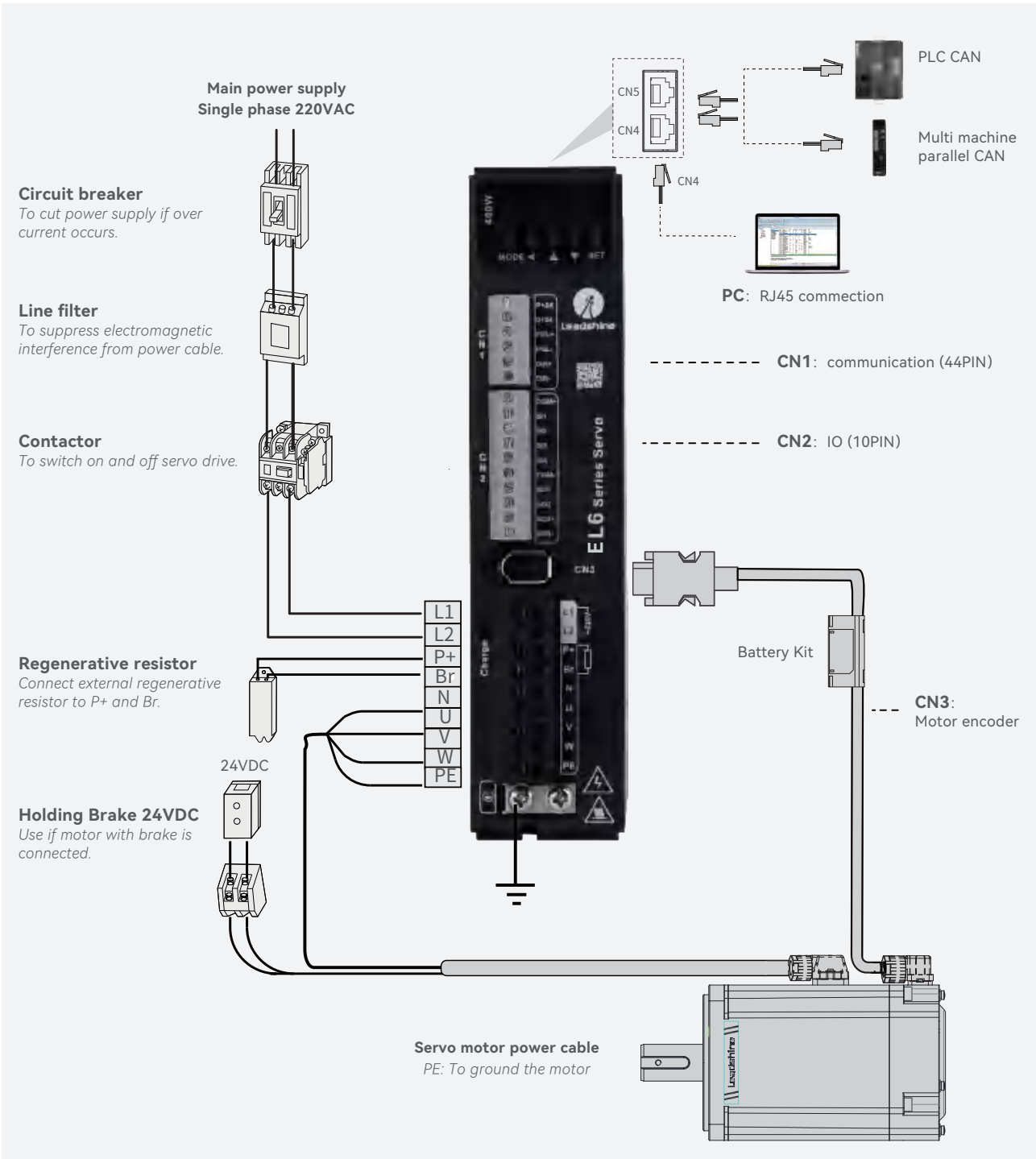
EL6-CAN & Peripheral Wiring Diagram
