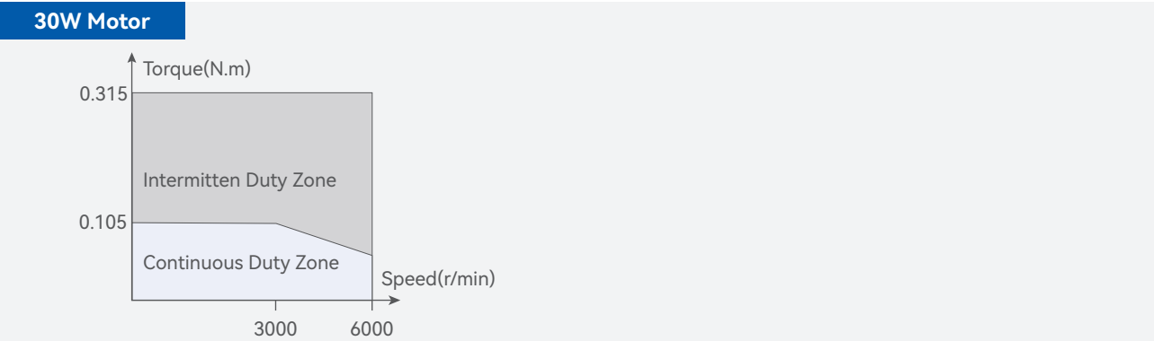
Speed-Torque characteristics
