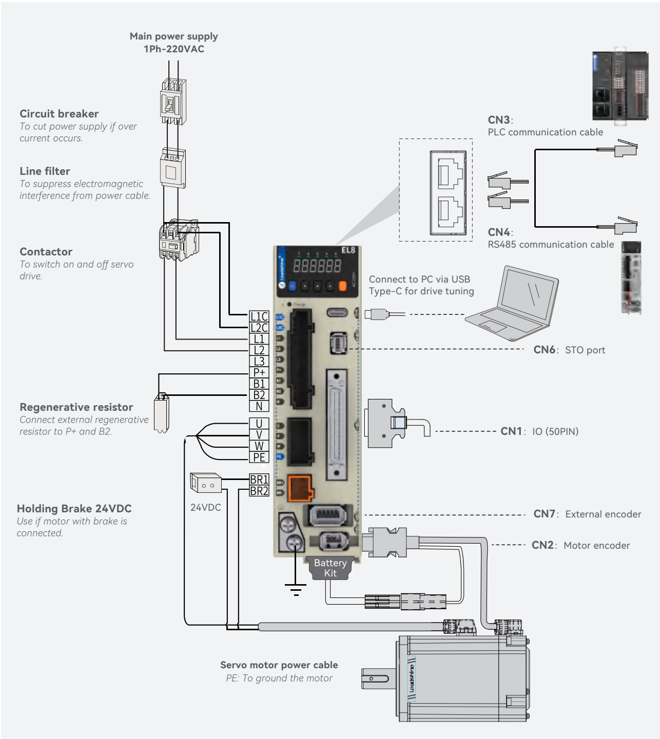
EL8-RS & Peripheral Wiring Diagram
