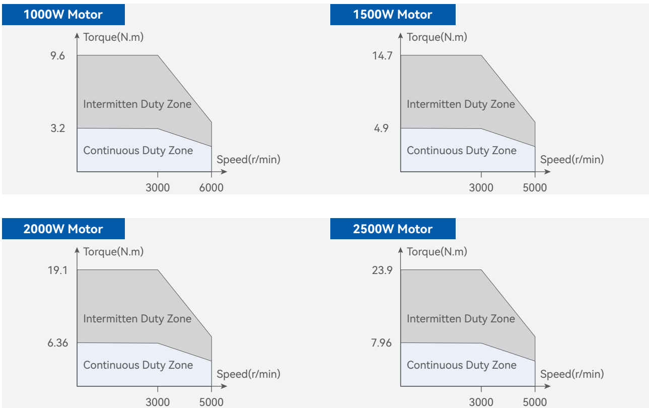
Speed-Torque characteristics
