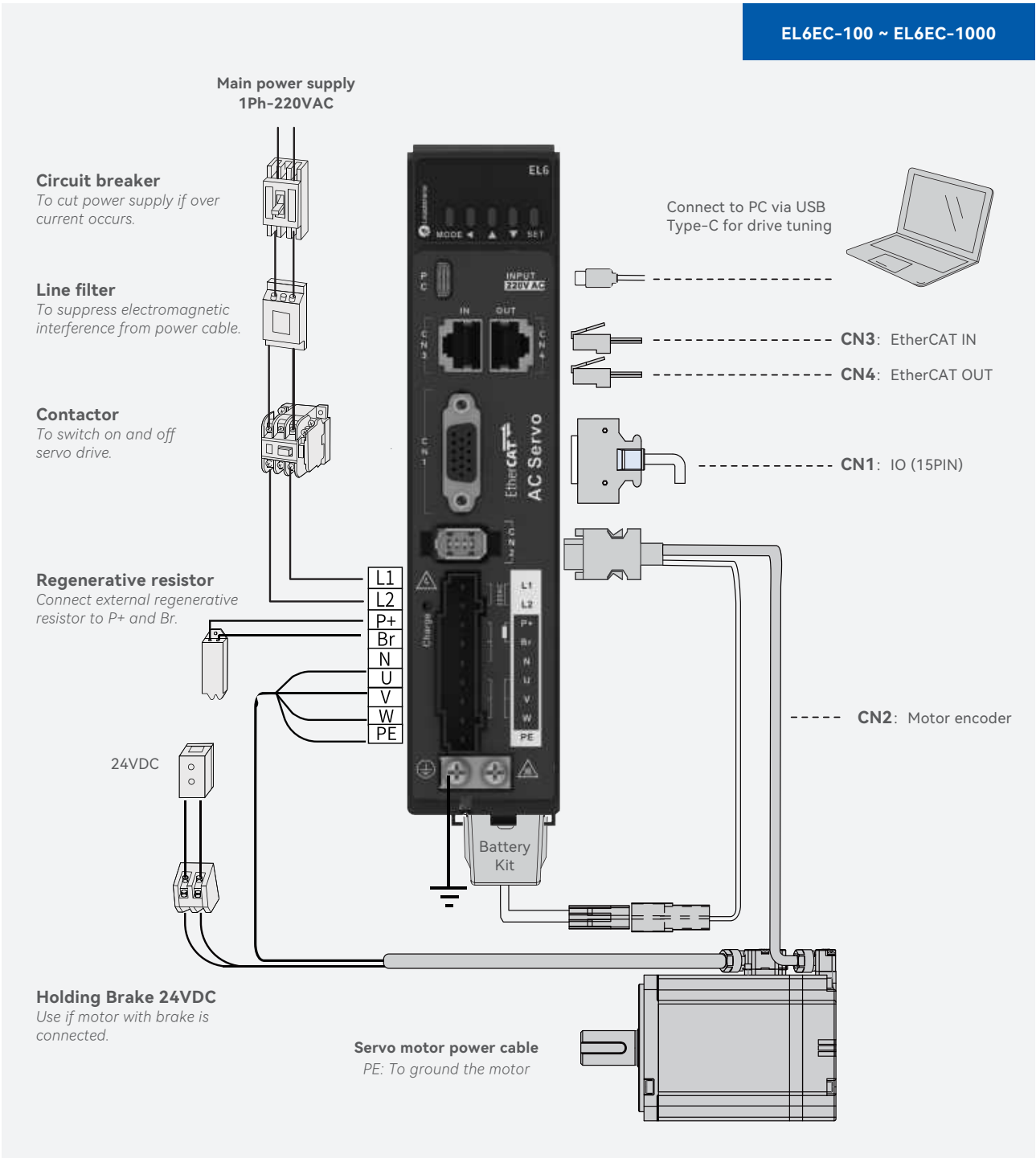
EL6-EC &amp; Peripheral Wiring Diagram
