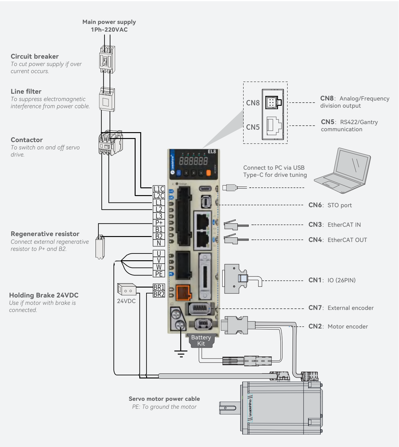
EL8-EC & Peripheral Wiring Diagram
