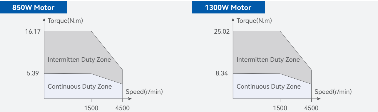
Speed-Torque characteristics
