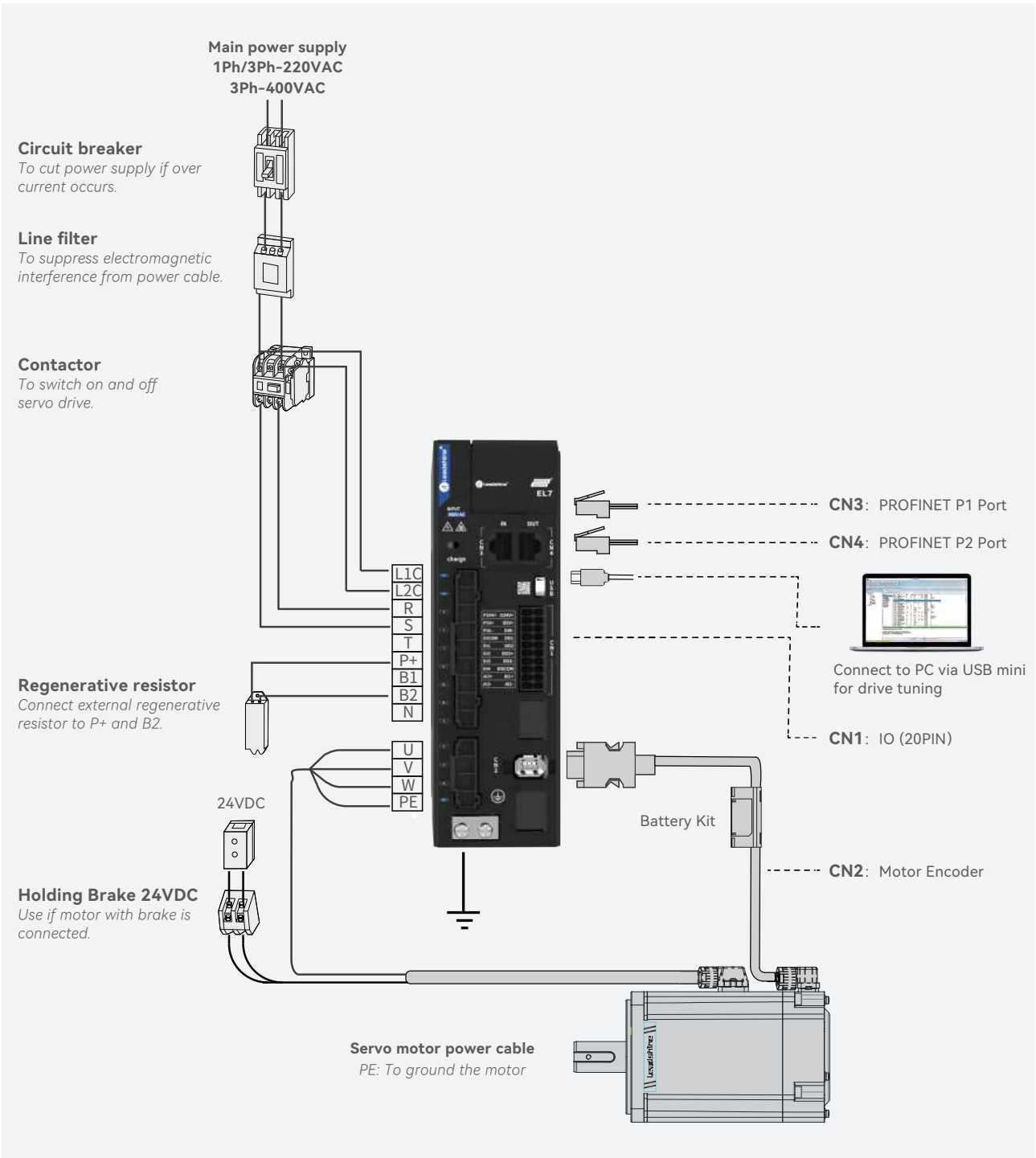
EL7-PN & Peripheral Wiring Diagram
