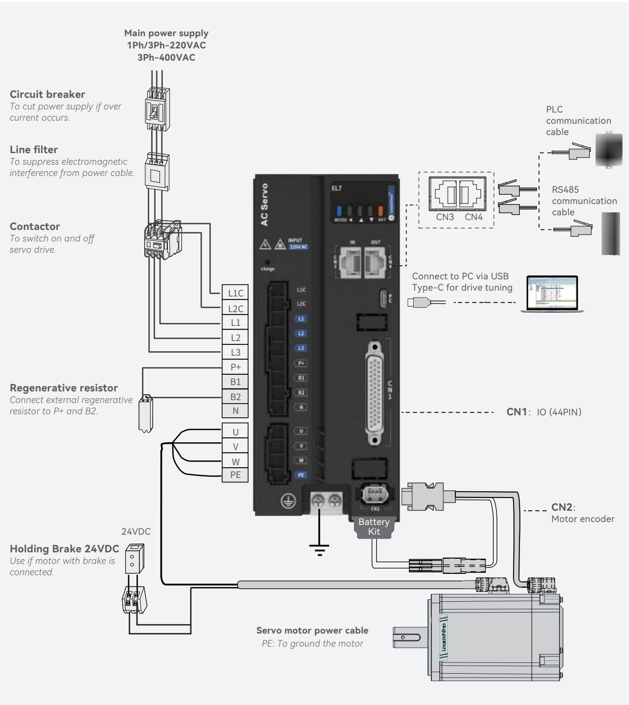
EL7-RS & Peripheral Wiring Diagram
