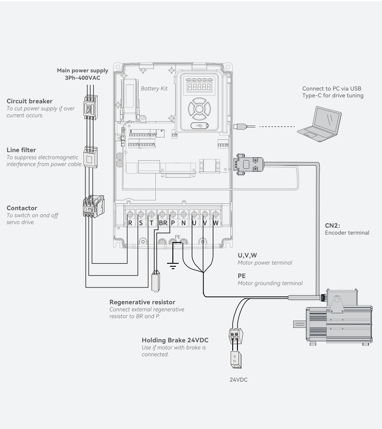
EL7-EC/RS (11-22kW) & Peripheral Wiring Diagram
